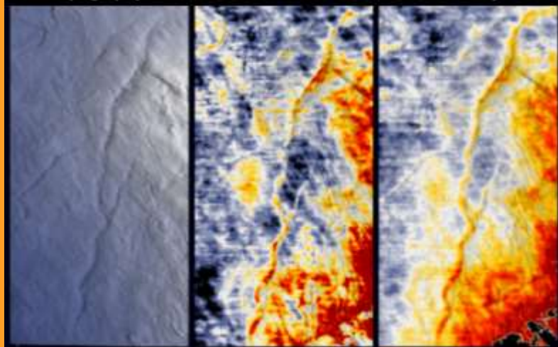
Topography Net:Gross Net Pay
